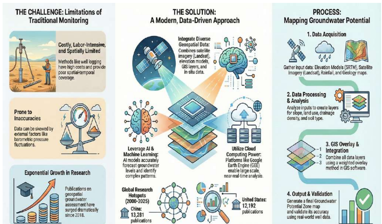
Fig. 3 Delineation of Groundwater Potential Zones (GWPZs) using RS (Remote Sensing), AI & ML Technology (Source: Prakash et al., 2025a)
