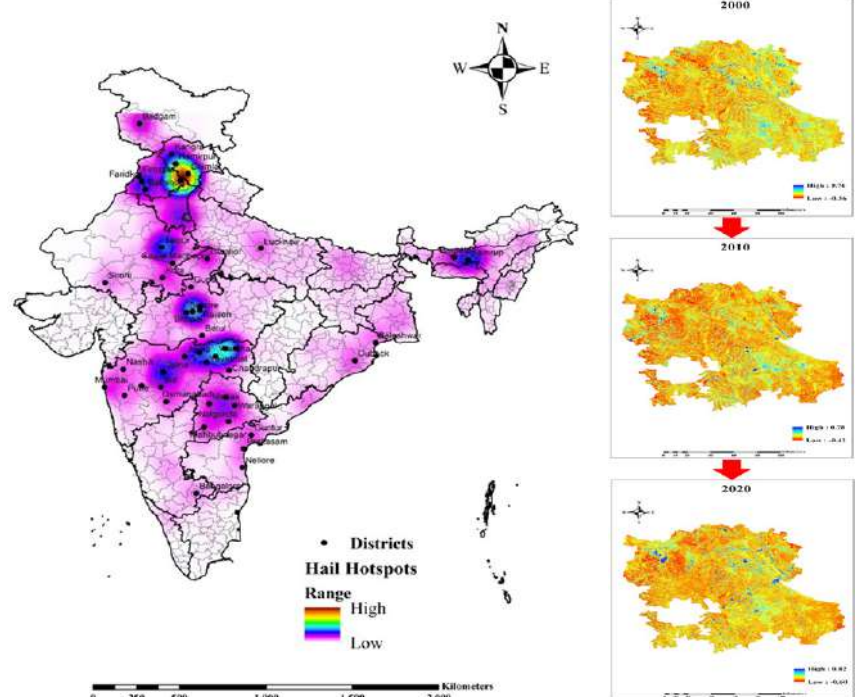
Fig. 4 The Hailstorm hotspots of India delineated using Kernel Density estimation revealed that among the states, Himachal Pradesh recorded maximum hail events spread over the majority of the months despite Maharashtra (614) being the highest hailstorm observed state of the country during the study period 1975 to 2020 (Source: Subba Rao et al., 2025)
